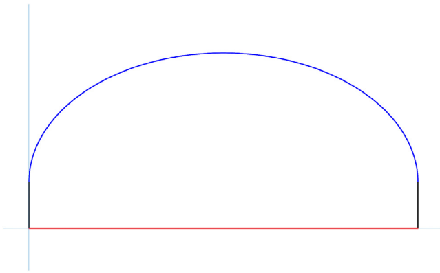
Fig. 1. Dorodnitzyn's diffeomorphism (\ell, s) is well defined in D .
